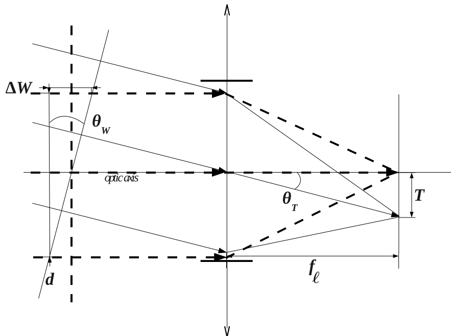
Figure 17: Shack-Hartmann Subaperture Geometry
