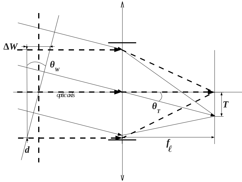
Figure 3: Tilt sensor
