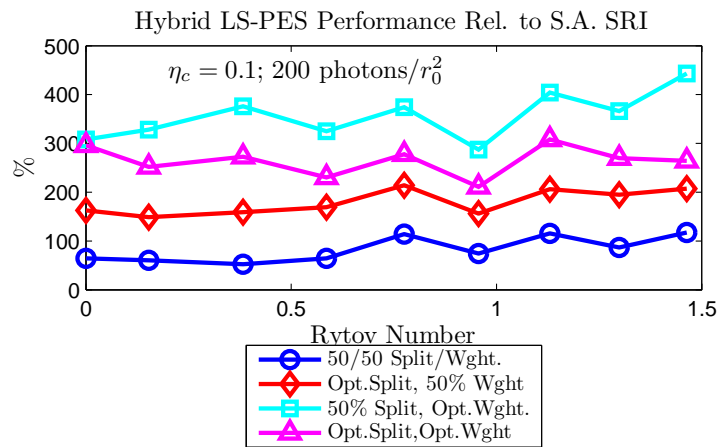
Figure 52: Hybrid's LSPES improvement over SRI LSPES Improvement of Hybrid WFS relative to stand-alone SRI for four approaches to optimizing.
