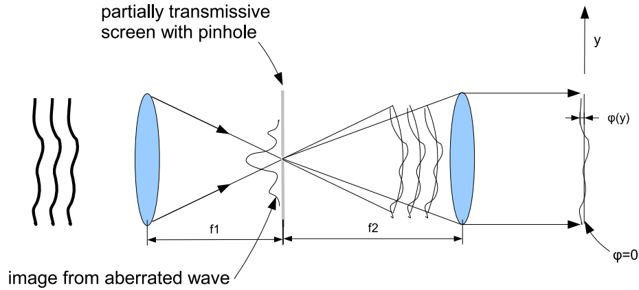
Figure 7: Point-diffraction interferometer.
