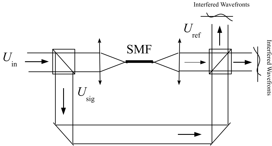
Figure 8: Self-Referencing Interferometer.
